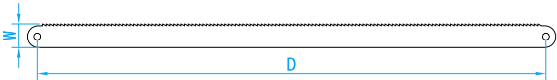
SIDE VIEW
